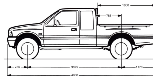
Sportscab
