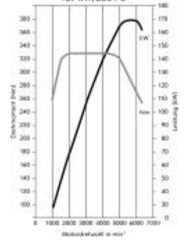
2.8 V6 Turbo ECOTEC® 169 kW/230 PS
