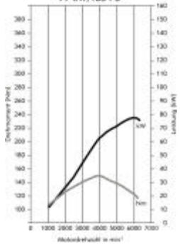
2.8 V6 Turbo ECOTEC® 169 kW/230 PS
