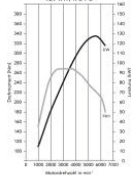
2.0 Turbo ECOTEC® 129 kW/175 PS
