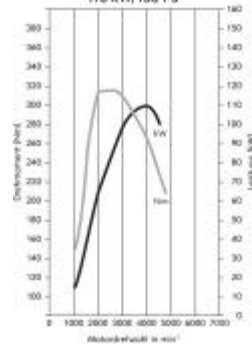
1.9 CDTI ECOTEC® 110 kW/150 PS
